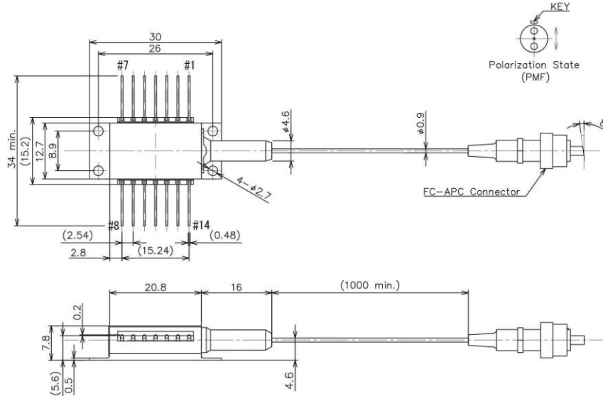
All dimensions in millimeters.
